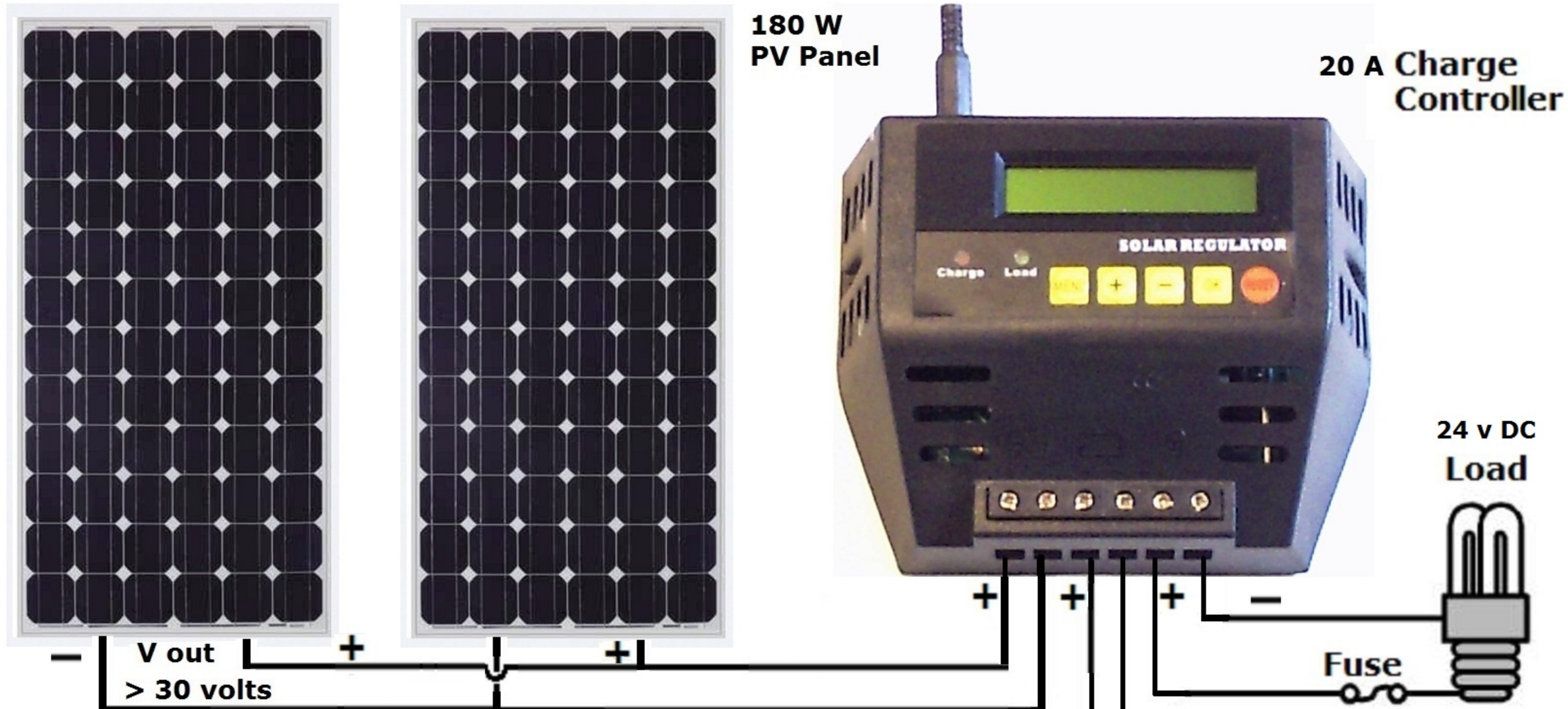
Wiring Diagram for chk24360
